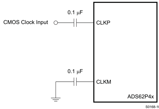
Figure 91. Single-Ended Clock Driving Circuit
