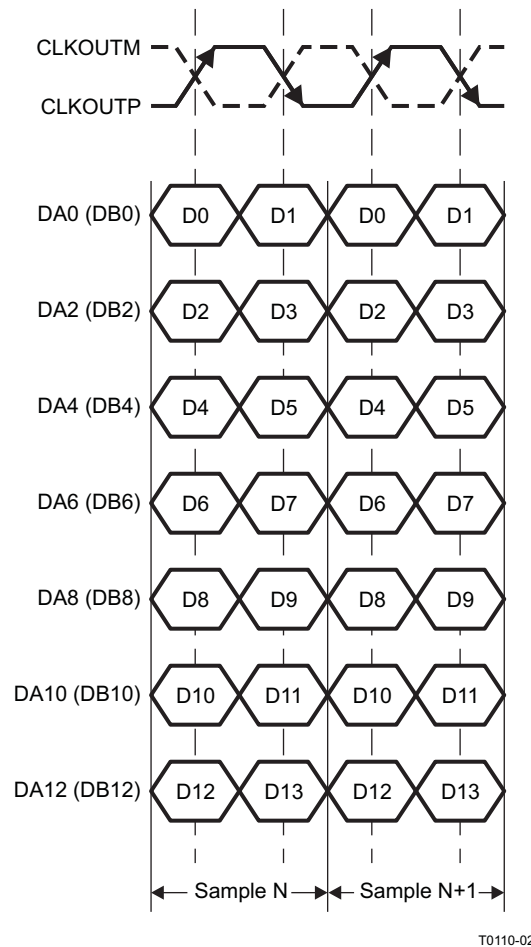
Figure 94. DDR LVDS Interface
